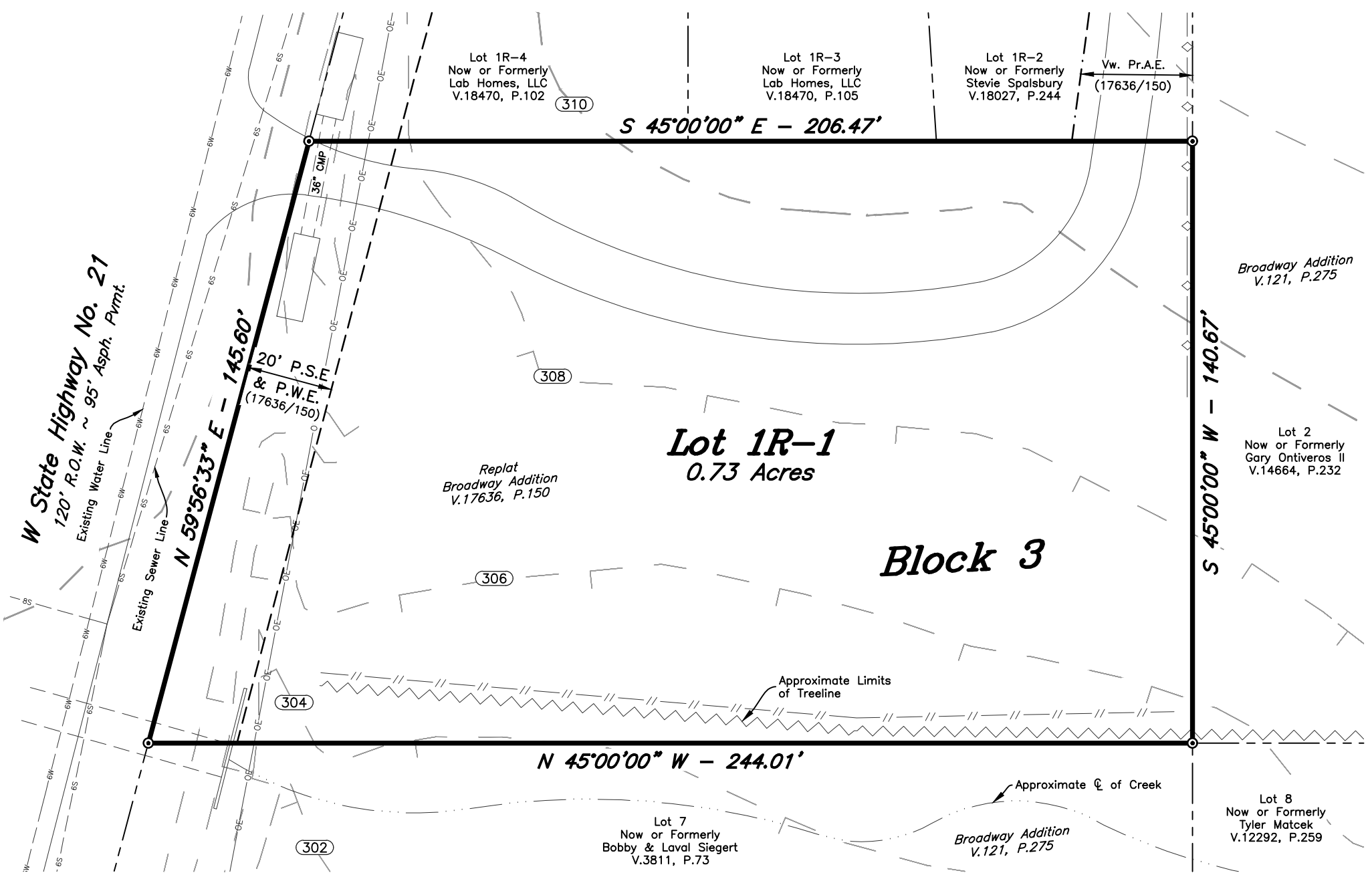
ORIGINAL PLAT LOT 1R-1, BLOCK 3, BROADWAY ADDITION AS RECORDED IN VOLUME 17636, PAGE 150
